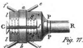
Aldersea's Engine for raising WATER
