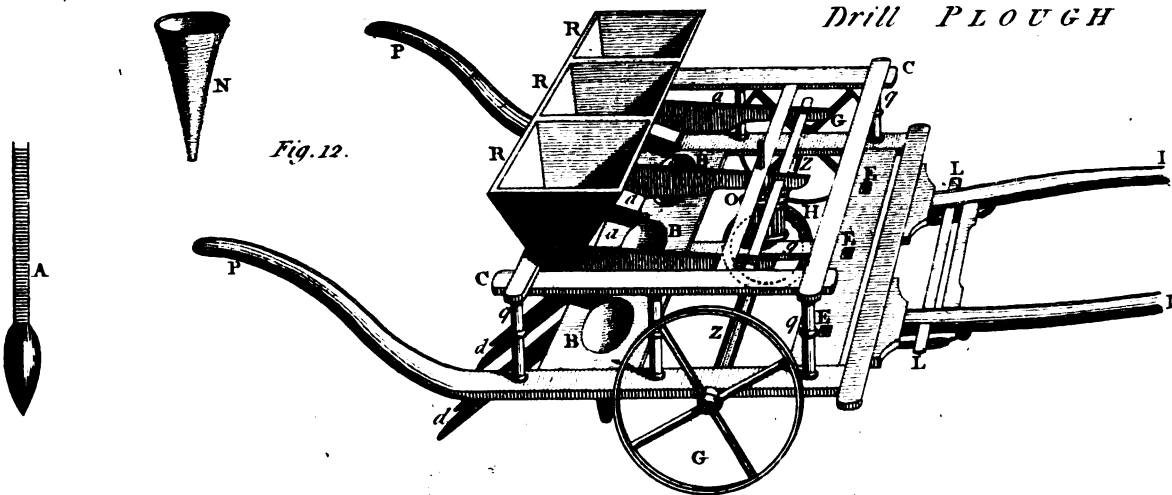
Four Coulter'd PLOUGH.
