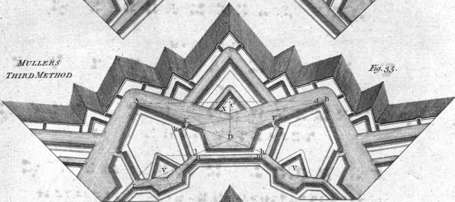
FORTIFICATION Irregular.
