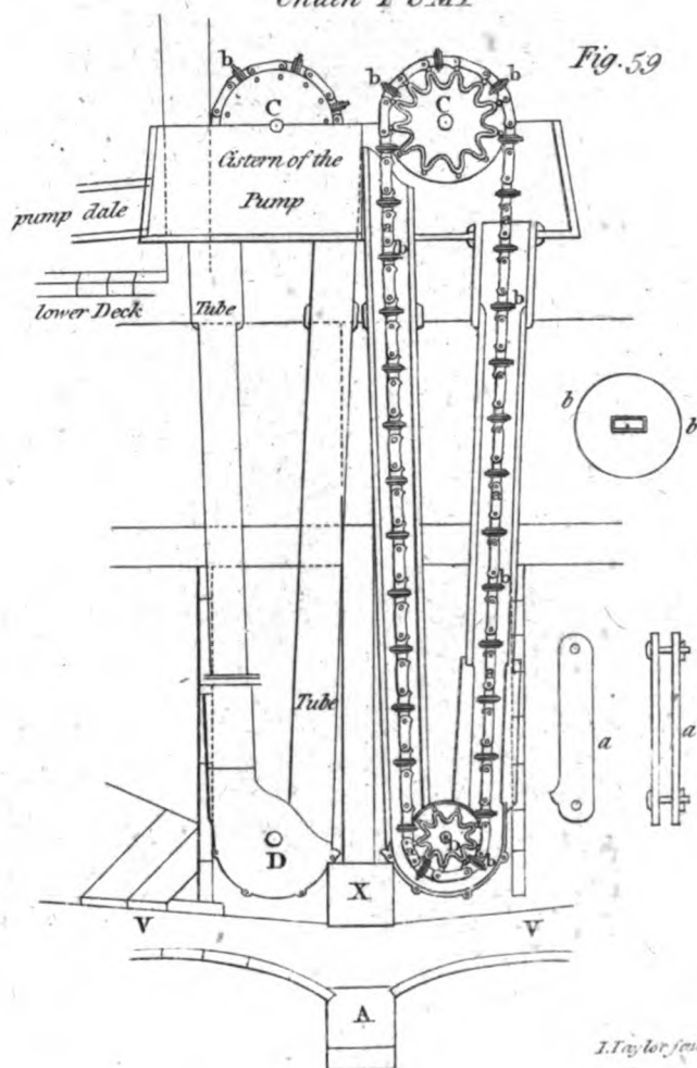
Chain PUMP
