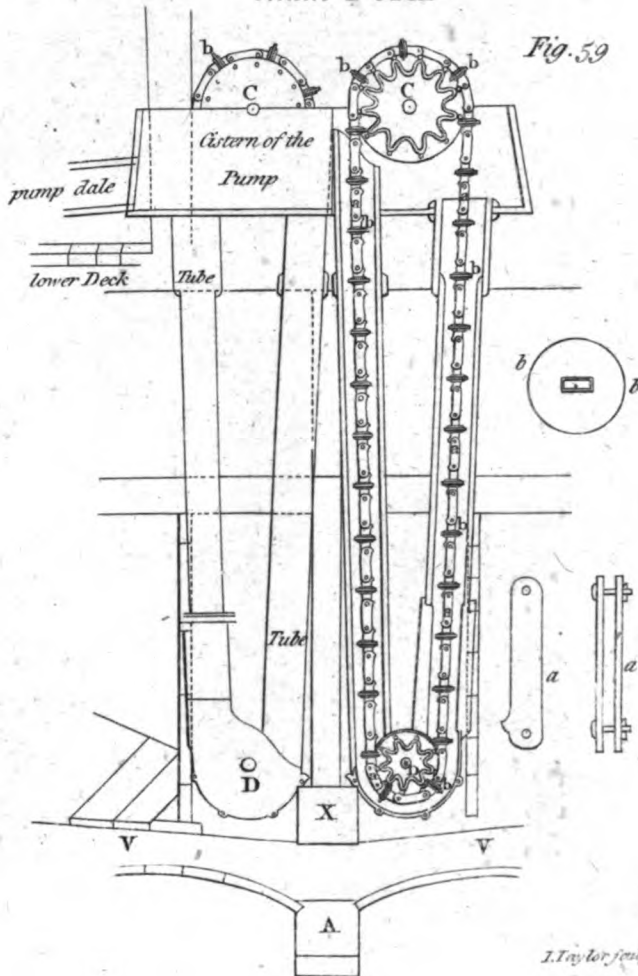
Chain PUMP
