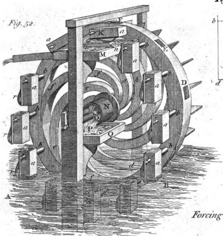
PERSIAN Wheel
