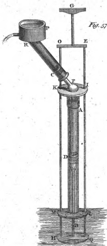
Lifting PUMP
