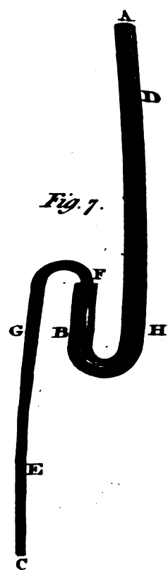
Rowning's BAROMETER
