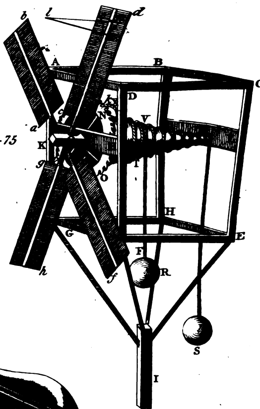
WIND - gun. Fig. 76.
