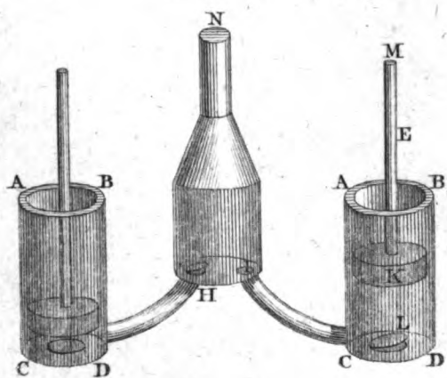
Ctesibes PUMP
