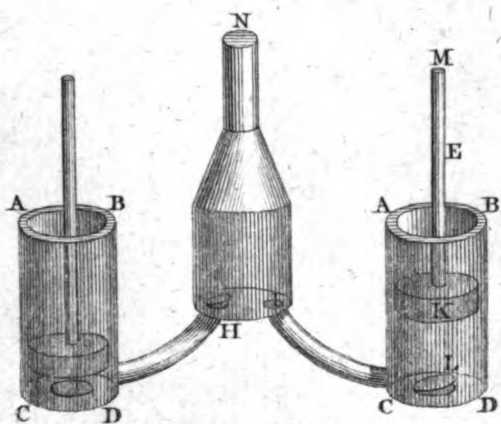
Ctesebes PUMP
