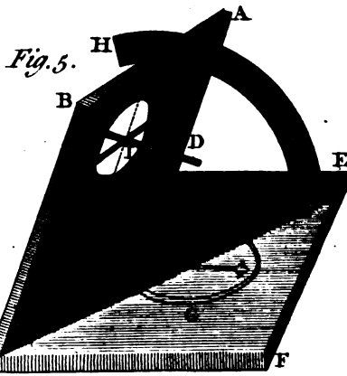
Universal Equinoctial DIAL
