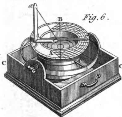
Azimuth COMPASS
