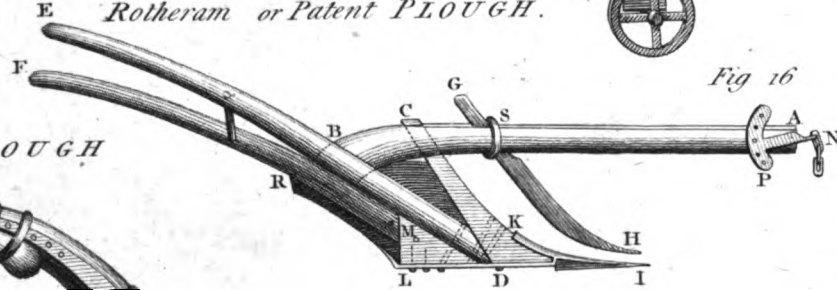
Rotheram or Patent PLOUGH.
