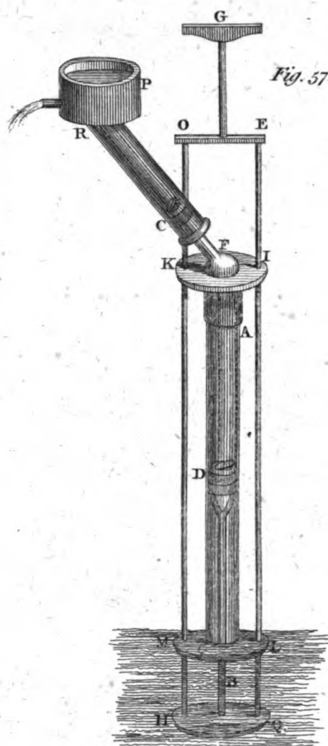
Lifting PUMP
