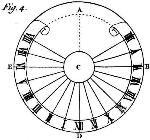
Equinoctial DIAL
