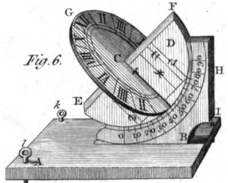
Universal DIAL
