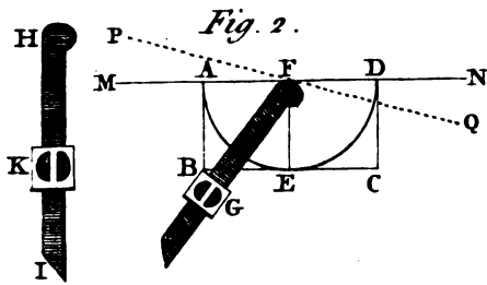
Universal Equinoctial DIAL
