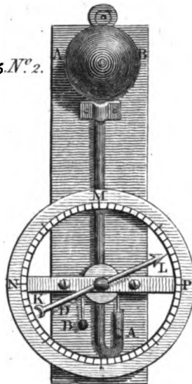
Wheel BAROMETER
