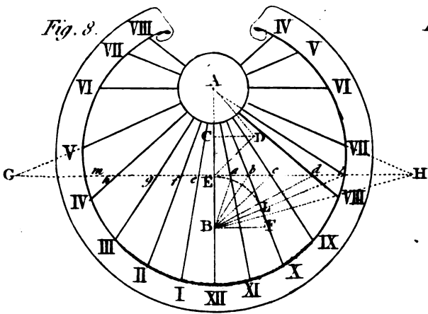
Horizontal DIAL
