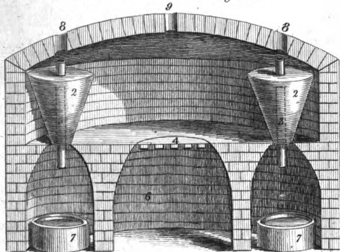
ZINC Furnace Fig. 59.
