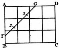
Mercator's CHART.
