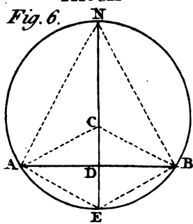
CIRCUMSCRIBING Polygon.
