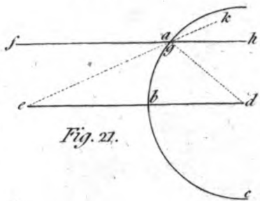
VIRTUAL FOCUS
