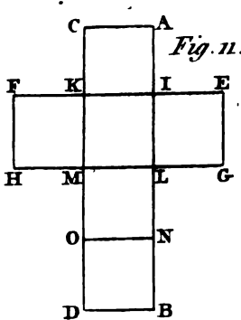
CUBE
