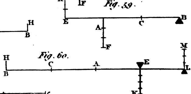
ACCELERATION
