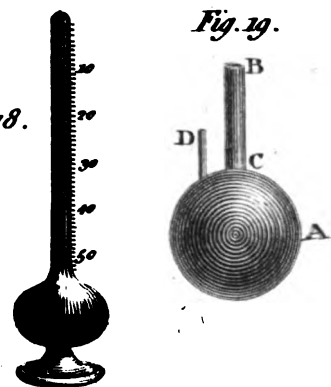
ATMOSPHERE
