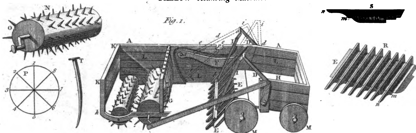
FALLOW cleansing Machine.
