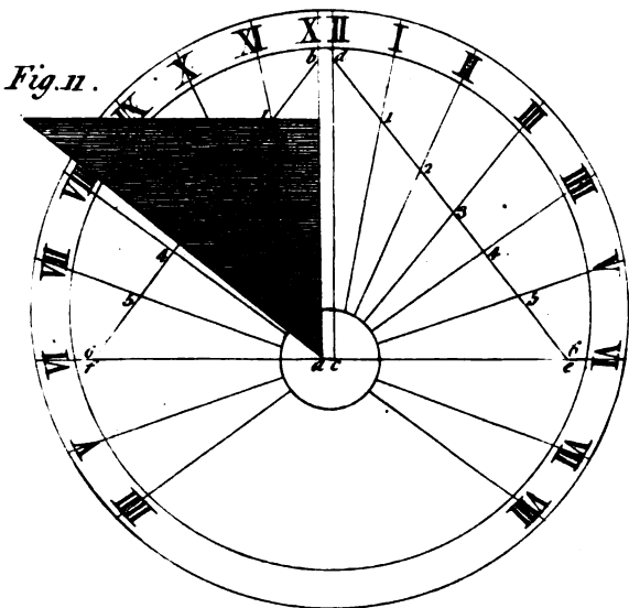
Vertical South DIAL
