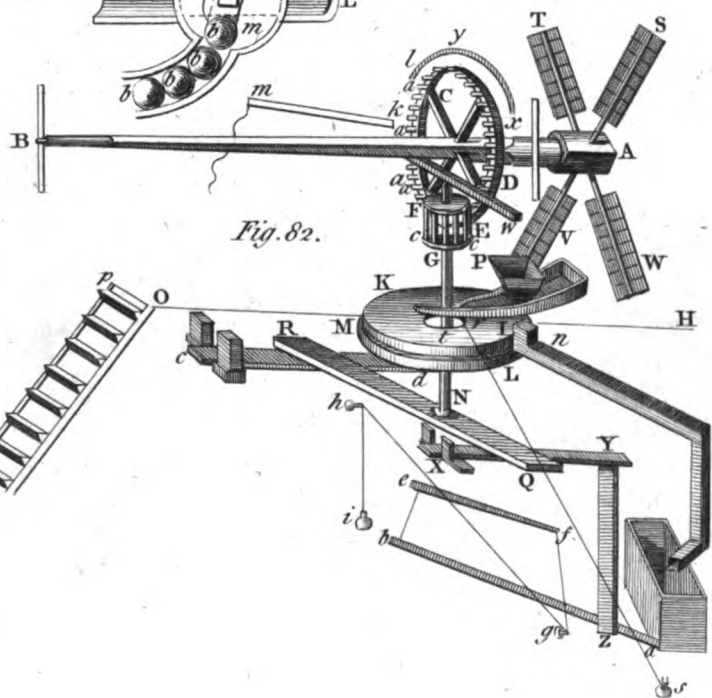
WIND - mill
