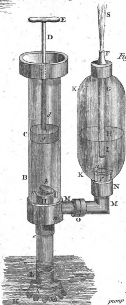
Forcing PUMP
