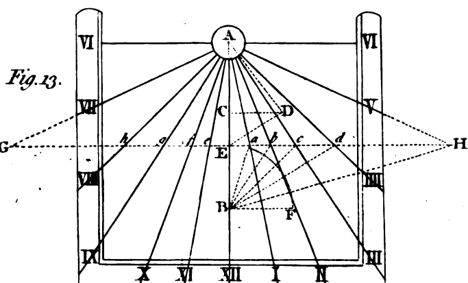
Vertical South DIAL
