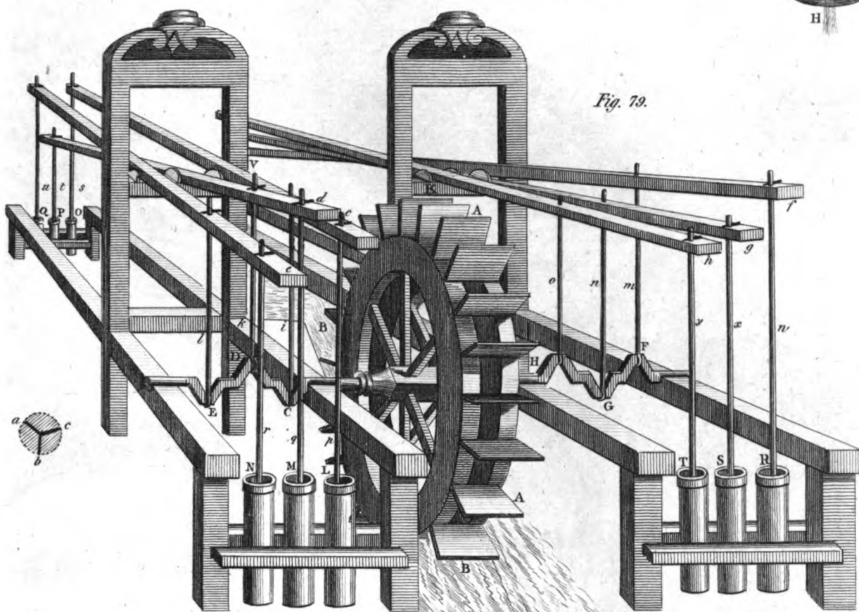
Aldersea's Engine for raising WATER
