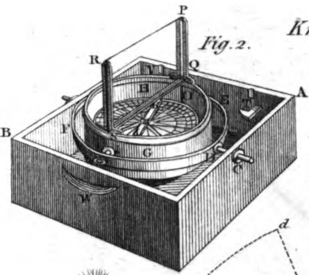
Azimuth COMPASS
