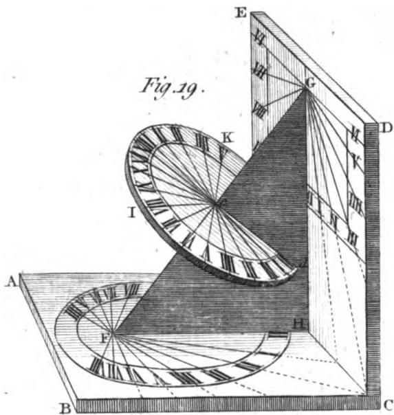
DIAL on three Planes
