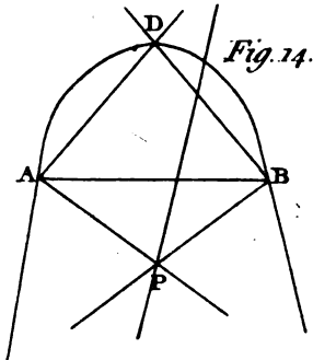
CYLINDER
