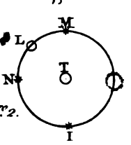
ARMILLARY Sphere
