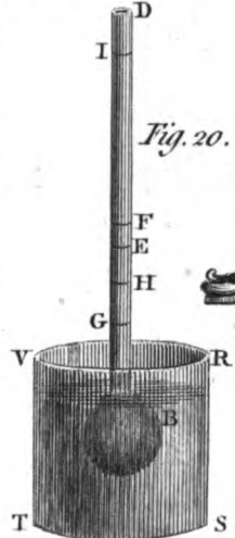
FREEZING
