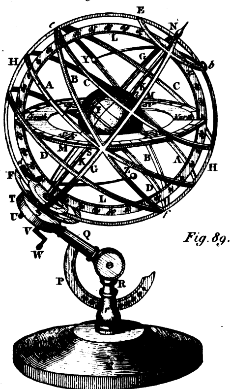
Armillary SPHERE
