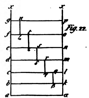
ATMOSPHERE
