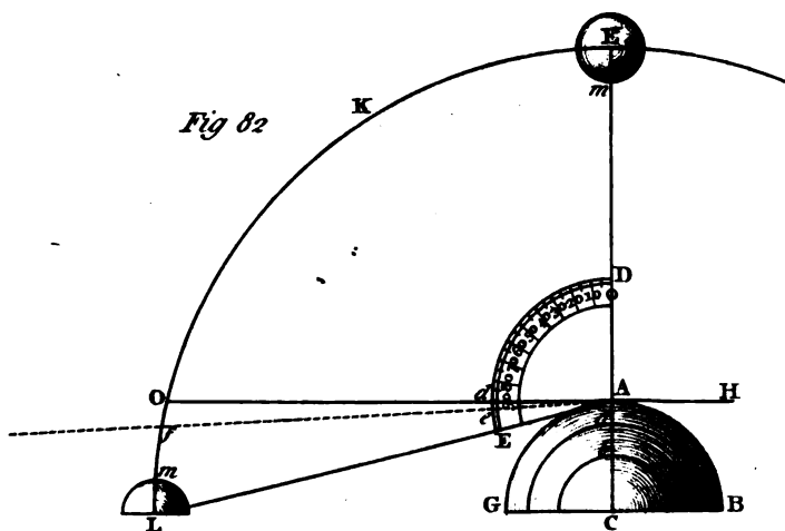
Moon's PARALLAX
