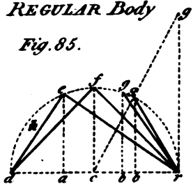
REGULAR Body
