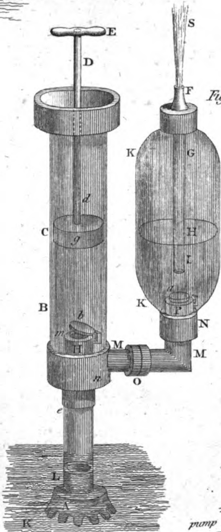
Forcing PUMP
