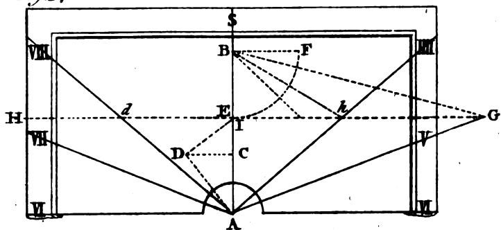
Fig. 14. Vertical North DIAL
