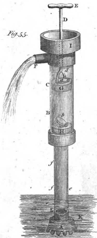
Sucking PUMP
