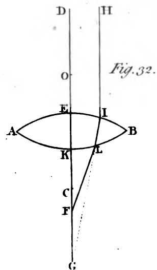
LENS
