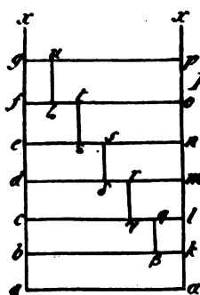
ATMOSPHERE
