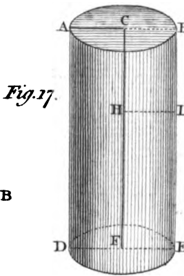
CYLINDER
