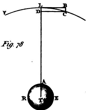
GRAVITY
