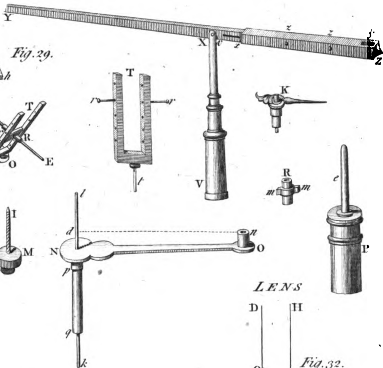
HOROPTER
