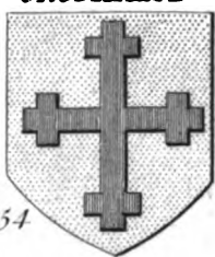
CROSSELET
