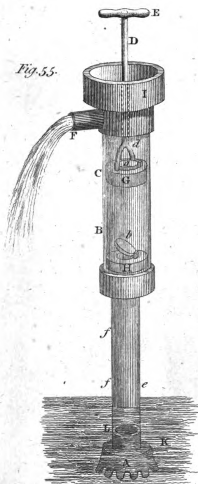
Sucking PUMP
