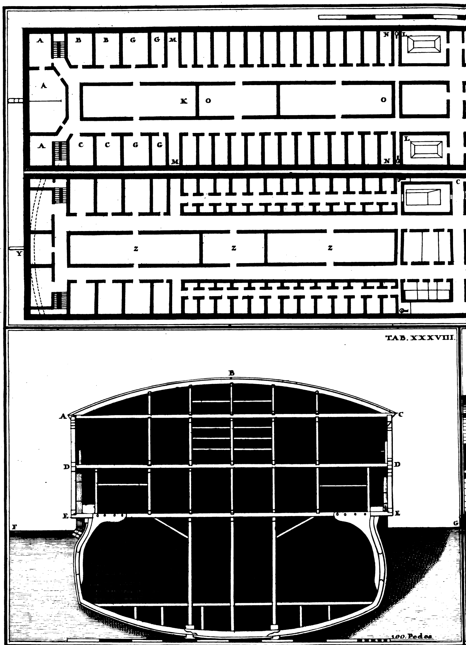
GENESIS Cap. VI. v. 15. Arcæ Ichnographia, Orthographia, Scenographia.
