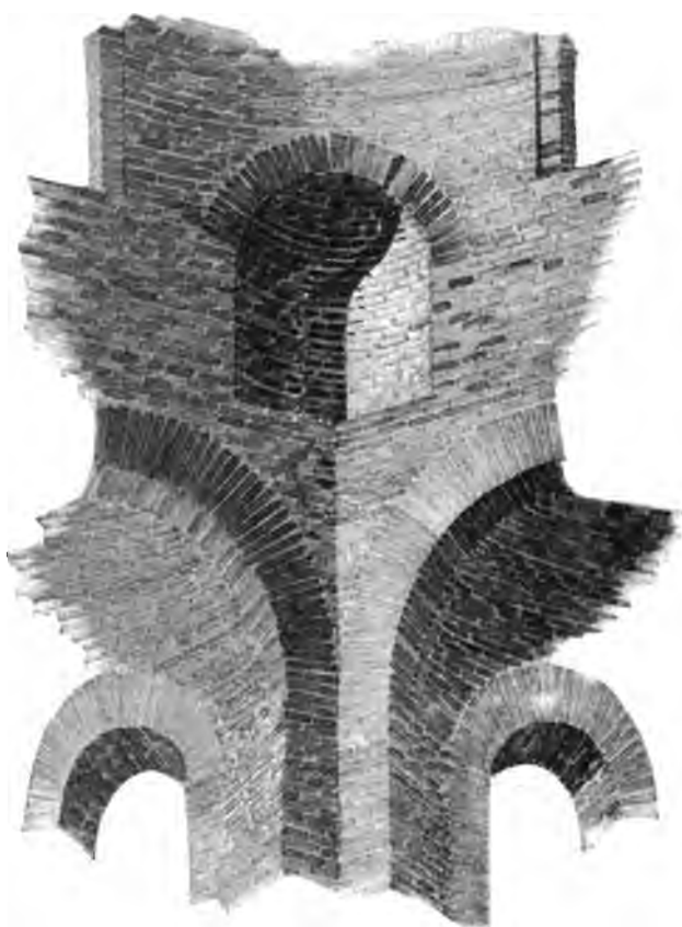
Fig. 82.—Ravenna. San Vitale. Pendentive of the Dome (526-547).
