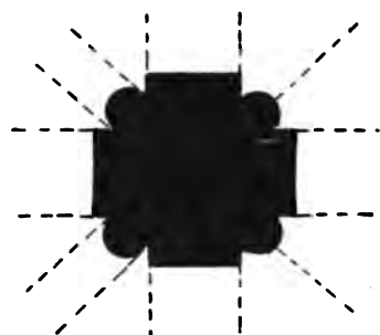
Fig. 332.—Rivolta d'Adda. Church of Santa Maria e San Sigismondo. Section of one of the large piers (XIth Century).
