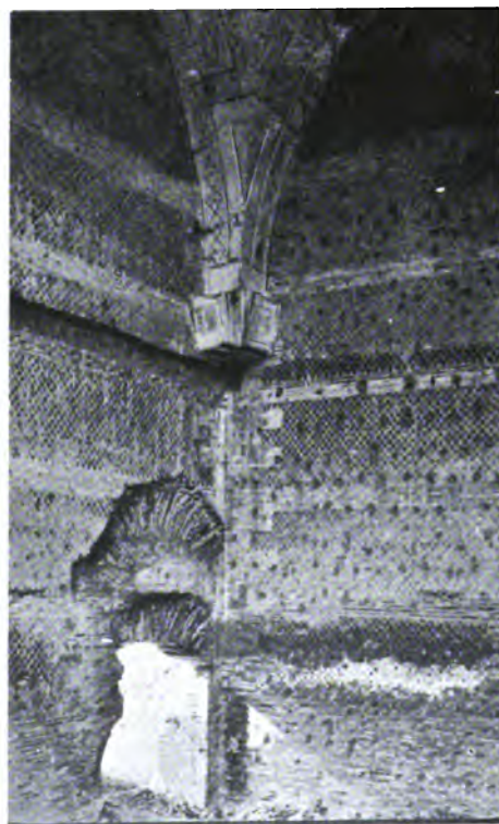
Fig. 120.—Tivoli. Villa of Hadrian. Hall in Great Baths (125-135).
