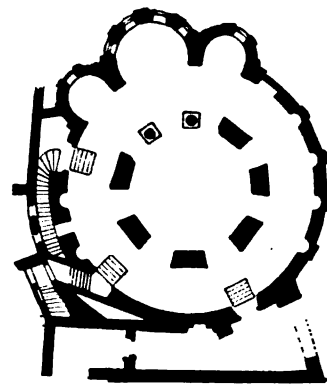
Fig. 210.—Zara. Ground plan of San Donato (about 801-806).
