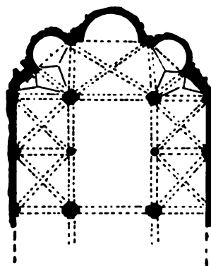
Fig. 301.—Montefiascone. Plan of San Flaviano (1032).
