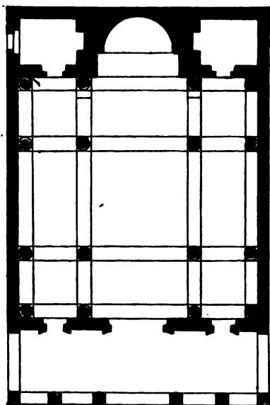
Fig. 24.—Plan of Church at Musmieh (IInd and IIIrd Centuries).
