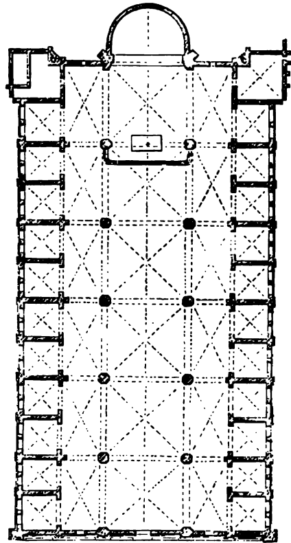
PLAN—SAN PETRONIO, BOLOGNA.
