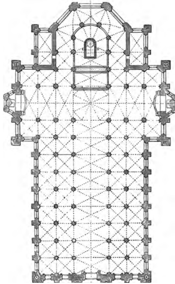
GROUND-PLAN—MILAN CATHEDRAL.
